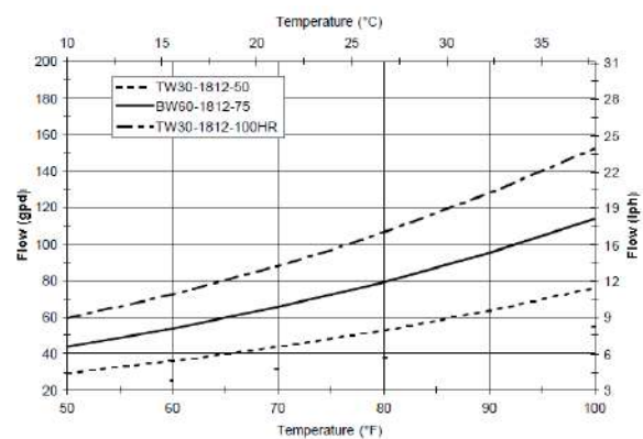
Figure 2: Impact of temperature on permeate flow (constant temperature, recovery)
