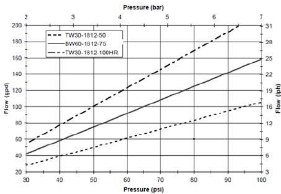
Figure 1: Impact of pressure on permeate flow (constant temperature, recovery)
